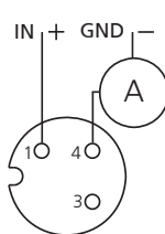
Current output
